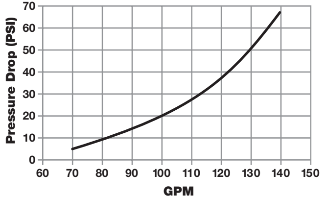
SS100 Pressure Drop Curve
