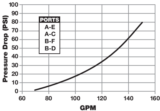
DS100 Pressure Drop Curve
